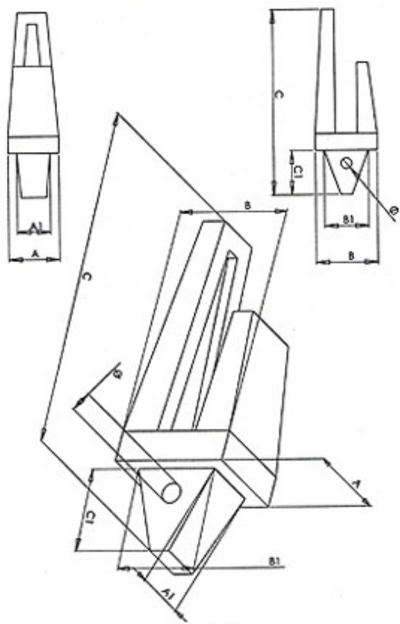
Drawing : Adapter(mm)
