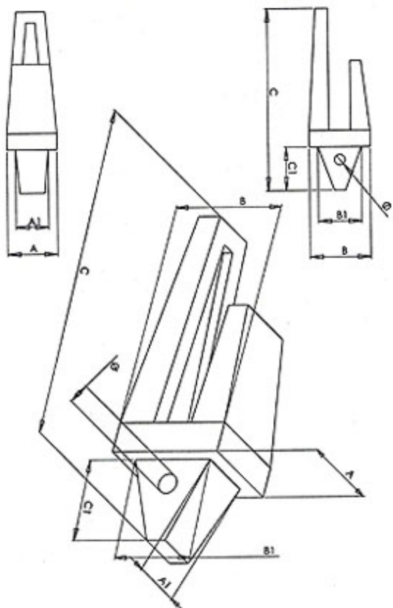
Drawing : Adapter(mm)
