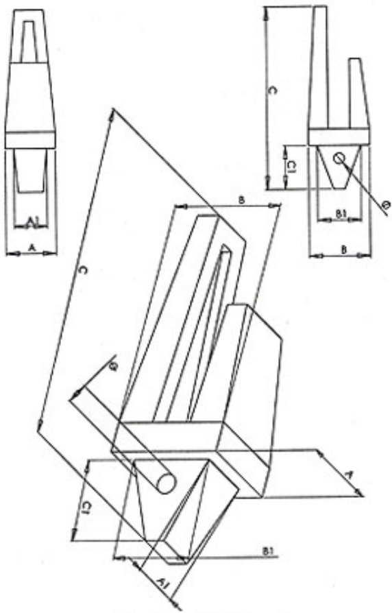
Drawing : Adapter(mm)
